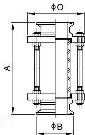
卡箍式直通视镜 Clamped straight sight glass
